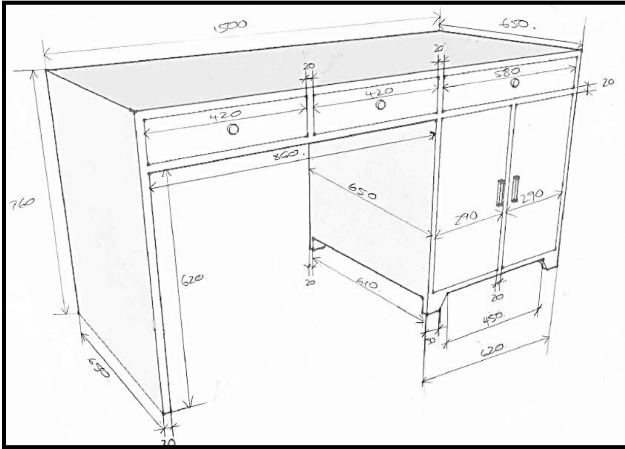
Drawing of cutting station with measurements
